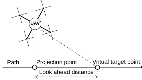
Fig. 2. Top view of the three dimensional path follower based on the carrot-chasing algorithm without taking into account the orientation error.
